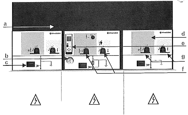
Figure 1.17: CGMCOSMOS-2LP cubicle synoptic
