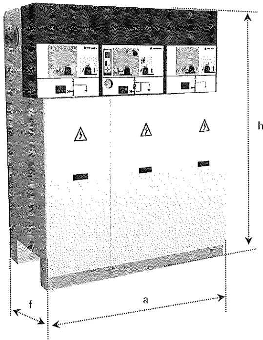
Figure 1.43: CGMCOSMOS-2LP cubicle dimensions
