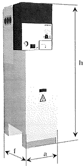
Figure 1.36: CGMCOSMOS-RB-Pt cubicle dimensions
