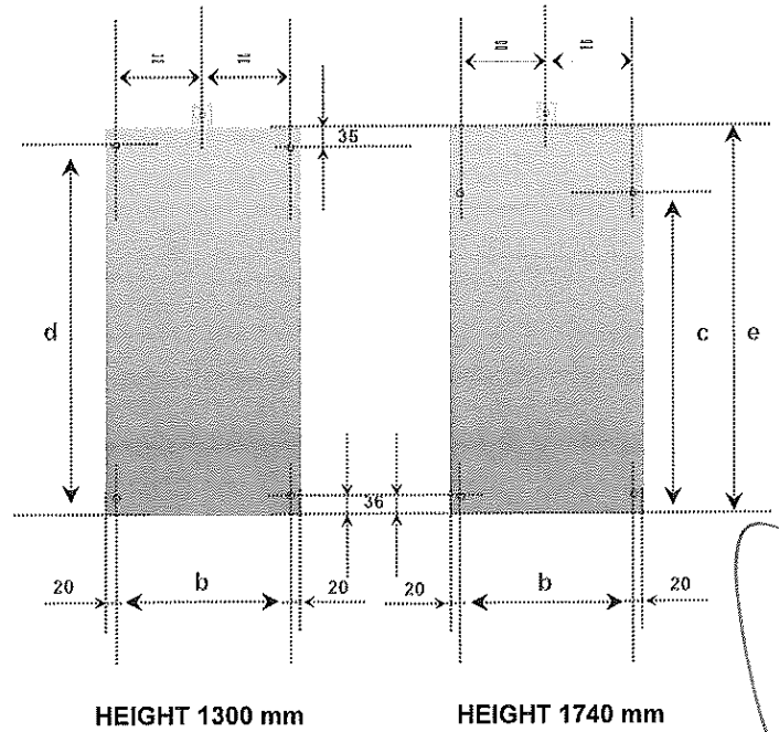
Figure 1.24: CGMCOSMOS-L cubicle anchorage points
